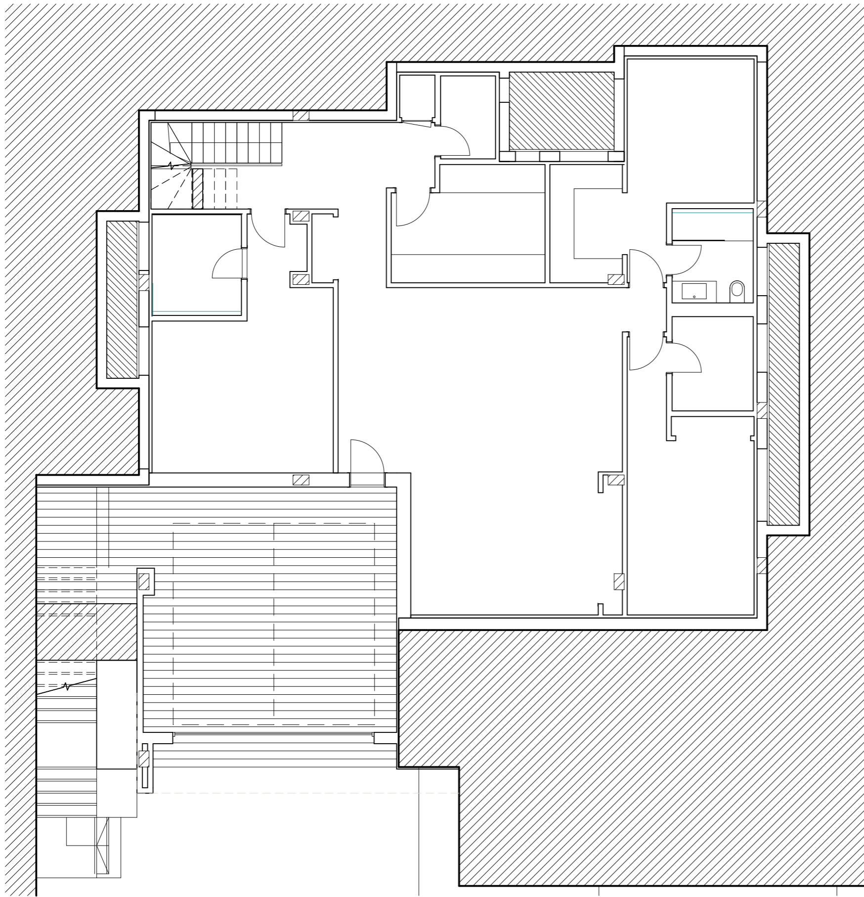
BASEMENT OPTION 2
