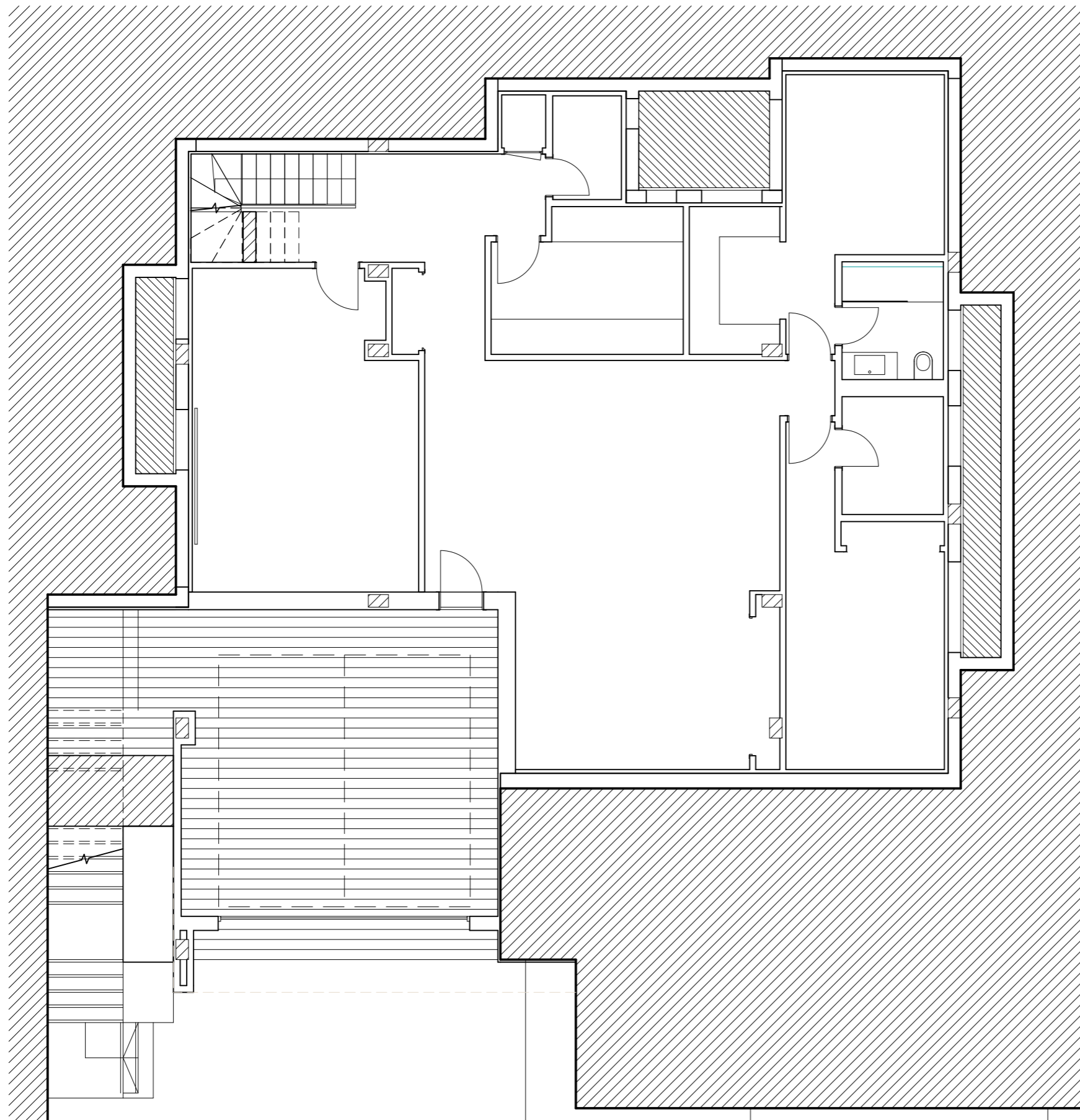
BASEMENT OPTION 1
