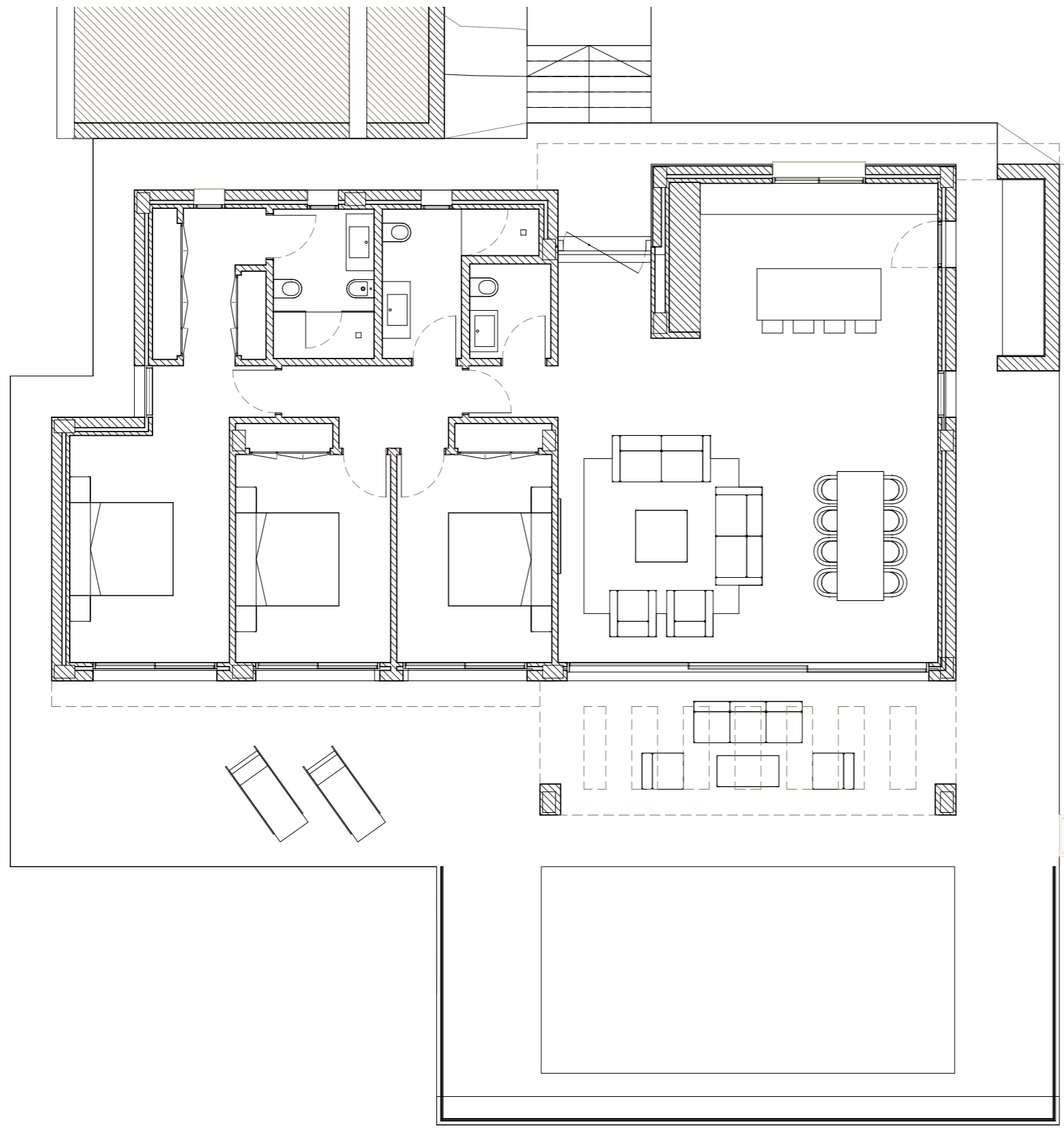
GROUND FLOOR
